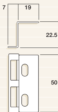
No hole outer pull W8227
