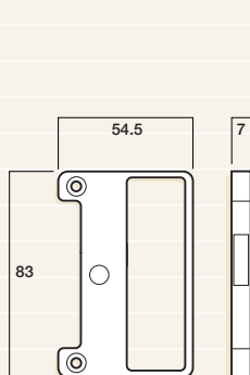
Outer pull with hole
