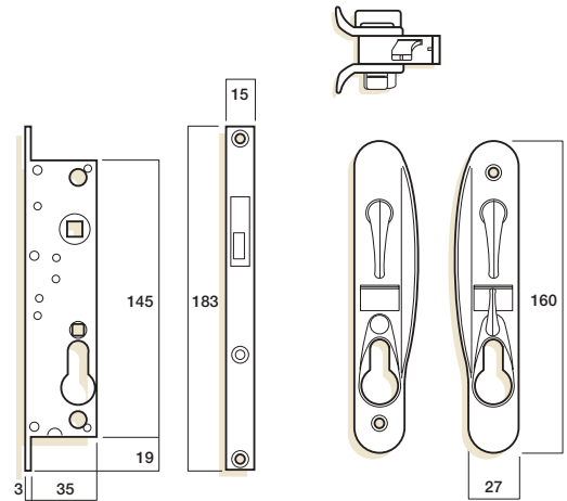
Cylinder locking
