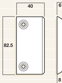
Standard Body W8215
