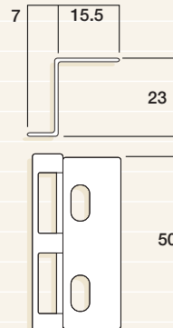
Short Snib W8221
